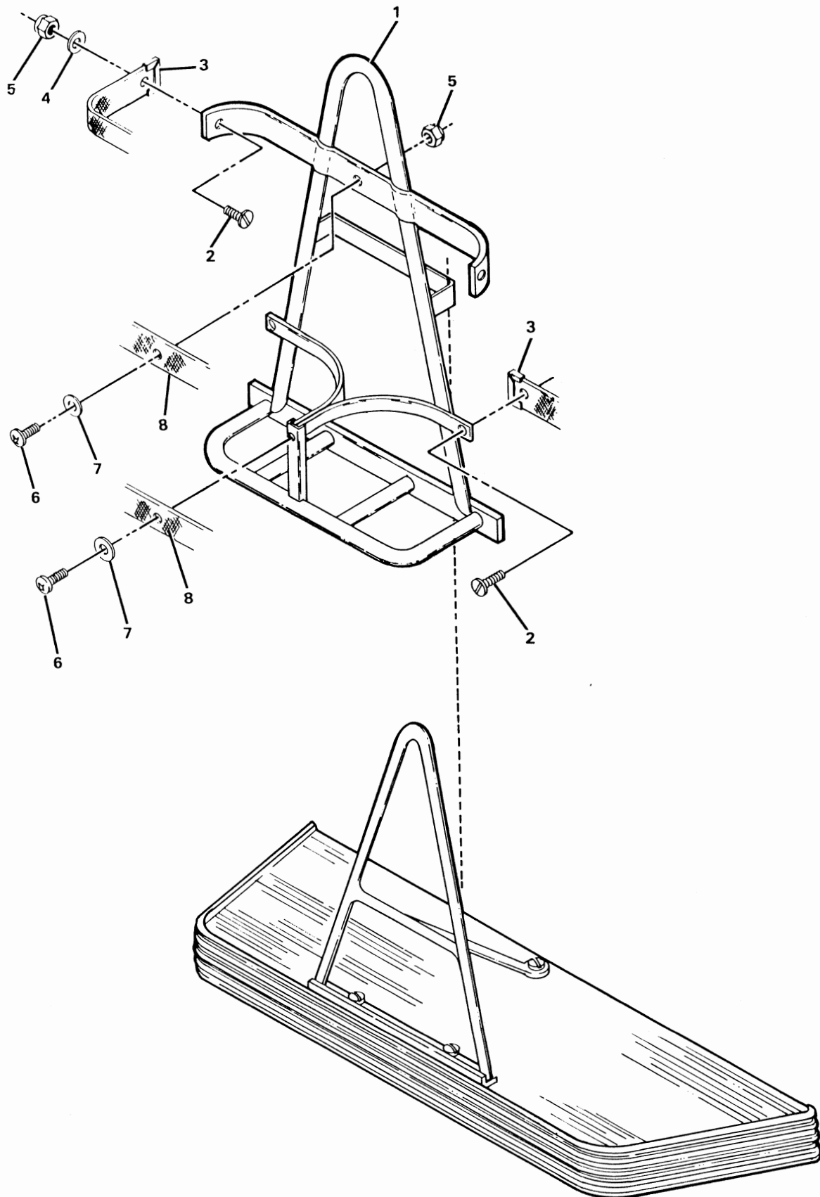
FIGURE 6-11. 4 BAG ATTACHMENT KIT (4-PASSENGER). SEE LIST 6-11.
