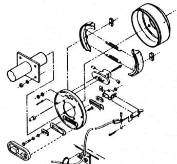
BRAKE CLUSTER ASS'Y, RIGHT HAND AND LEFT HAND FIGURE 4-1 PAGE 4-2
