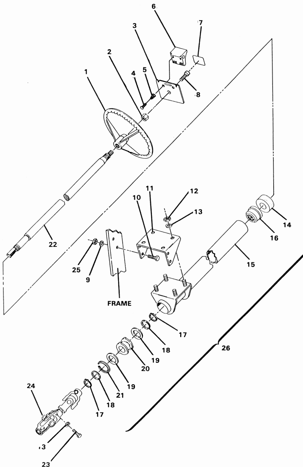
FIGURE 3-1. STEERING ASSEMBLY. SHEET 1 OF 2. INDEX NOS. 1-26. SEE LIST 3-1.
