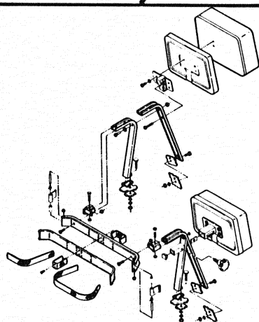
SEAT BACK & BAG HOOP ASS'Y FIGURE 1-3 PAGE 1-8
