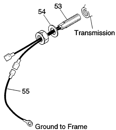
MAGNETIC PICKUP DETAIL
