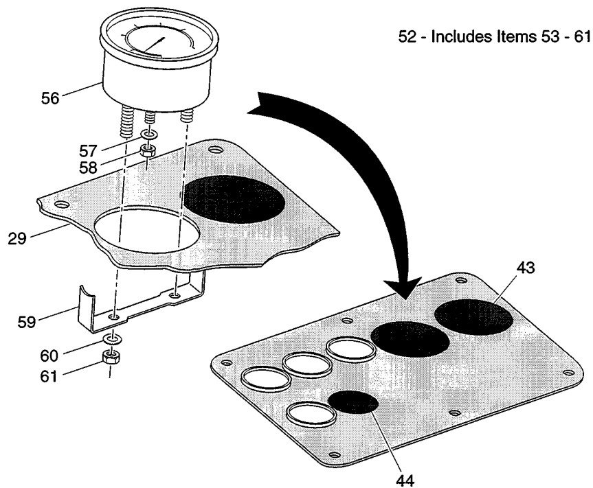
SPEEDOMETER DETAIL
