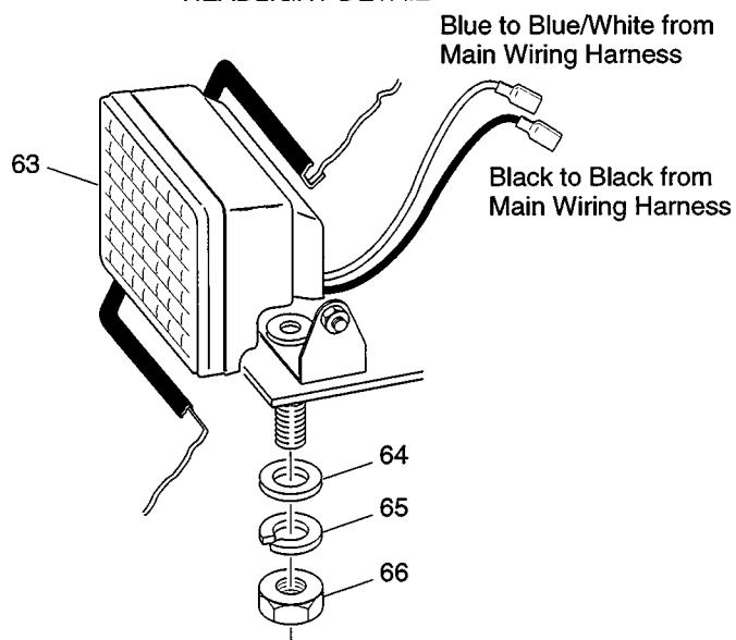
HEADLIGHT DETAIL
